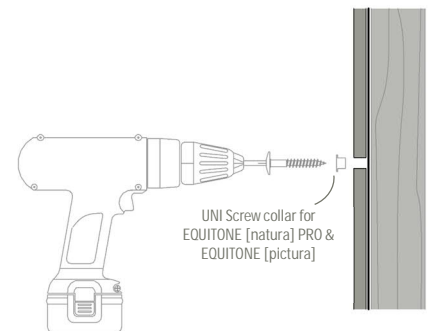
UNI Screw collar shall be used with EQUITONE [natura] PRO and EQUITONE [pictura]
