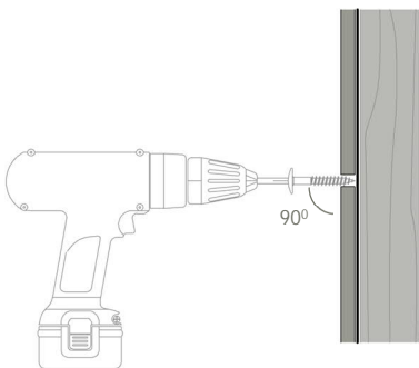
Ensure the screw is applied perpendicular to panel fac
