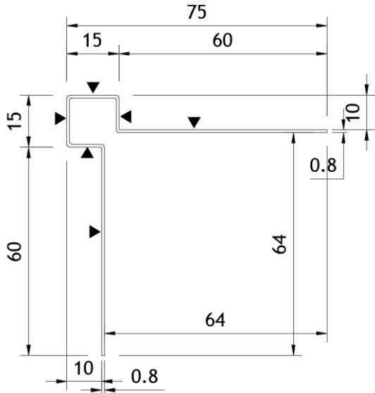
EQUITONE horizontal joint profile Art. N° 4031409
