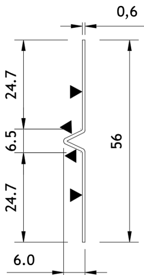
EQUITONE horizontal joint profile Art. N° 4031409
