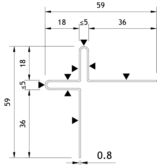
EQUITONE connection profile Art. N° 4031226
