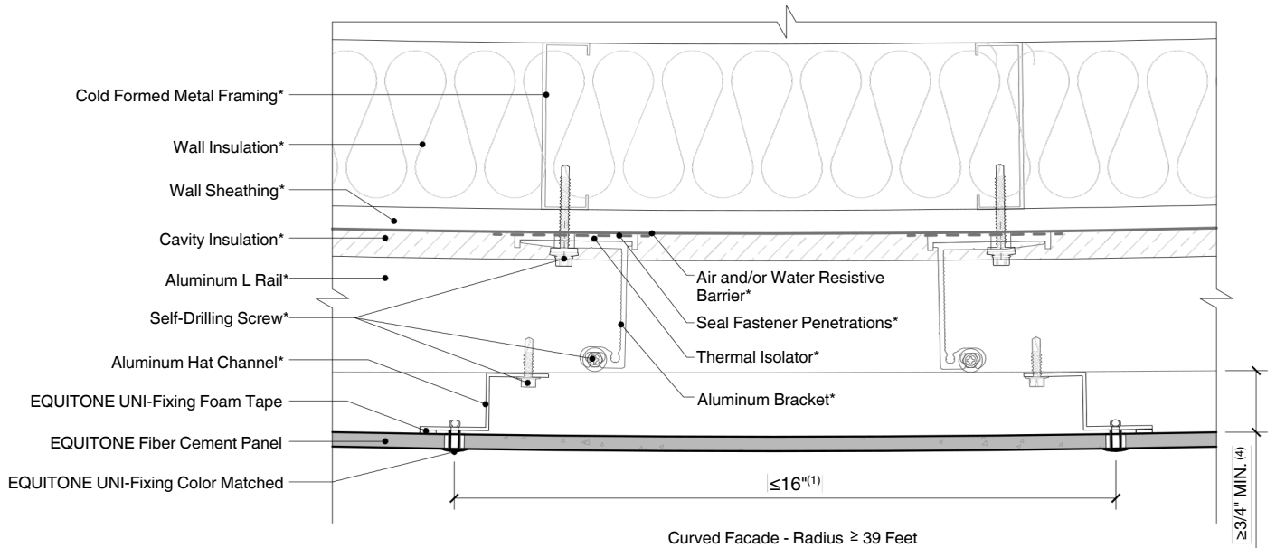
Curved Facade - Radius \geq 39 Feet
